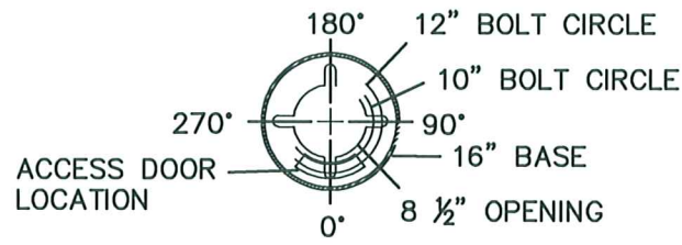
ANCHORAGE DETAIL
